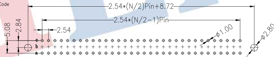
Recommended P.C.B Layout(Top Side) (PCB BOARD TOLERANCE±0.05)
