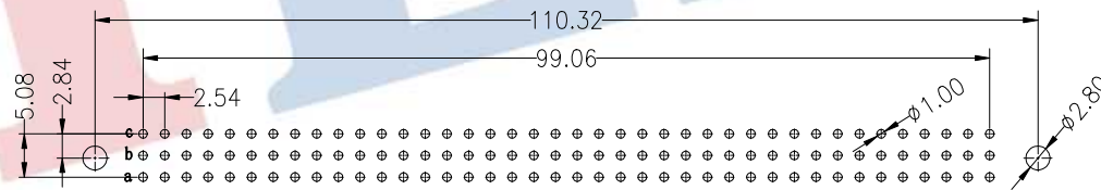
Recommended P.C.B Layout(Top Side) (PCB BOARD TOLERANCE± 0.05)
